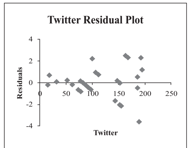
Figure 1: Residual plots of the linear models
