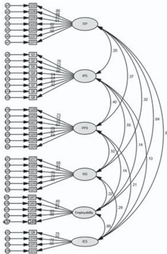
Figure 1: Output of Preliminary Model
