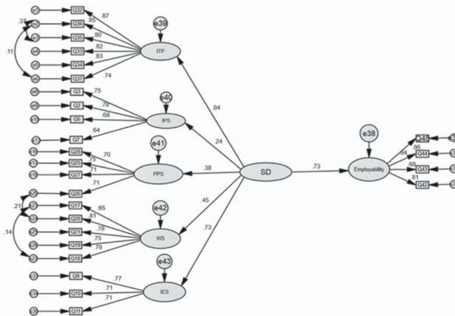
Figure 4: Revised (Standardized Regression Coefficients) Structural Model
