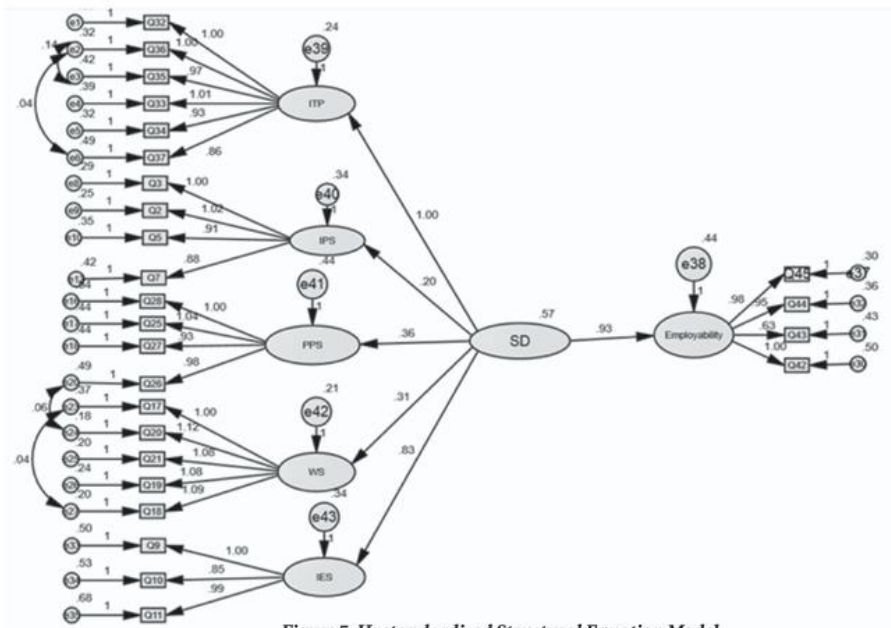
Figure 5: Unstandardized Structural Equation Model
