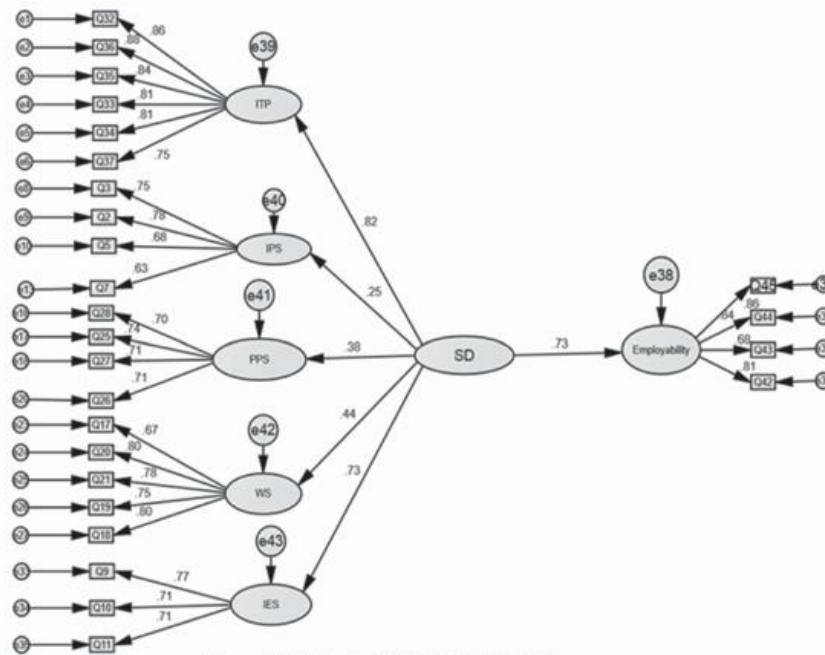
Figure 3: Output of Initial SEM Model
